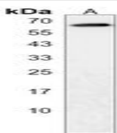
Western blot analysis of IFNGR1 expression in MCF7 (A) whole cell lysates.
