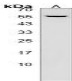
Western blot analysis of AP3D1 expression in U87MG (A), mouse kidney (B) whole cell lysates.
