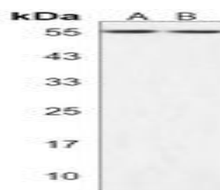
Western blot analysis of Ku70 (Acetyl-K338) expression in HeLa (A), NIH3T3 (B), PC12 (C) whole cell lysates.
