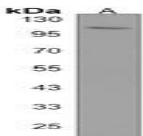
Western blot analysis of Histone H2A.X (Phospho-S139) expression in NIH3T3 treated with Hydroxyurea (A) whole cell lysates.
