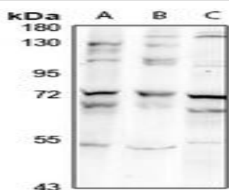
Western blot analysis of SMAD9 expression in HepG2 (A), A549 (B)
